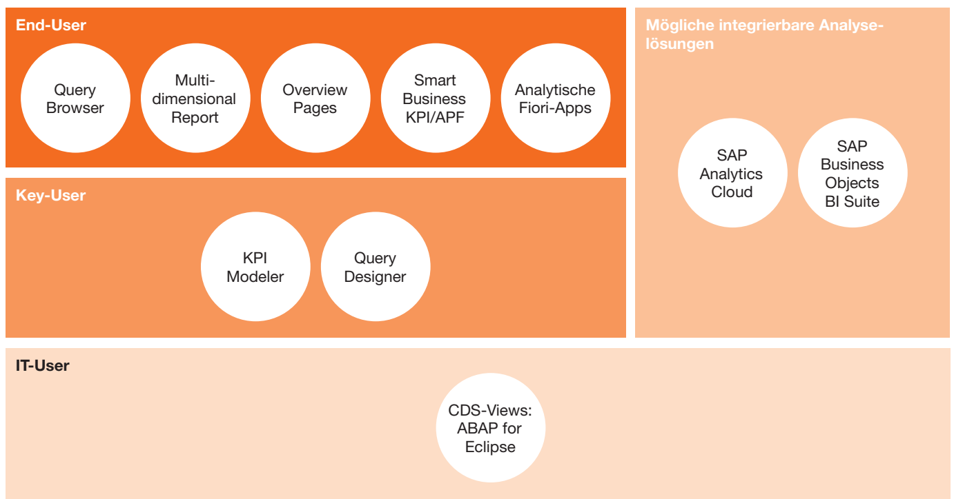
Abb. 2 SAP S/4HANA Embedded Analytics
