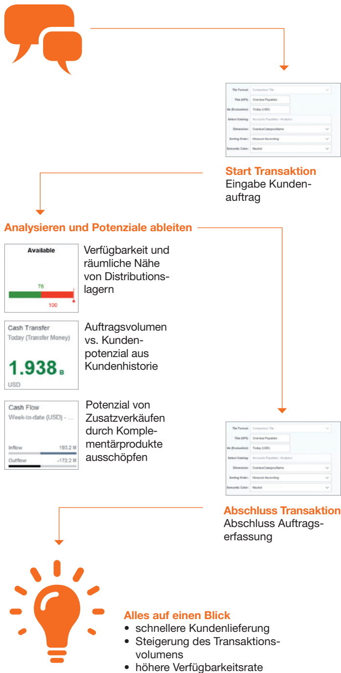
Abb. 1 Insight-to-Action-Prinzip
