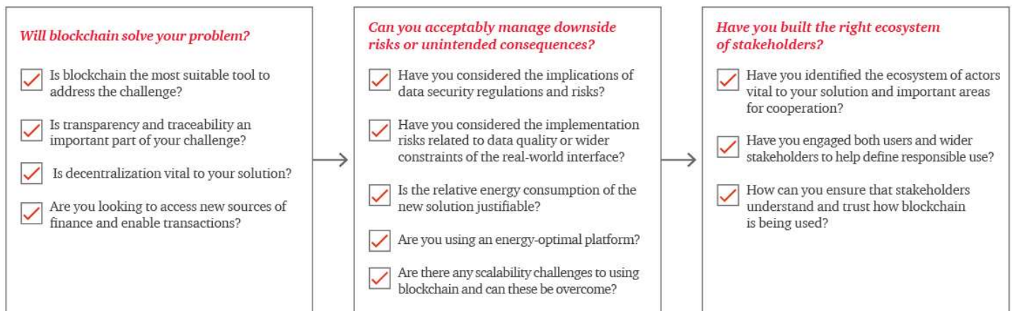
Figure 7: Blockchain principles
