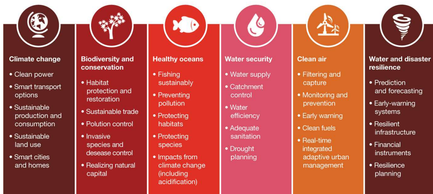
Figure 4: Priority action areas for addressing Earth challenge areas
